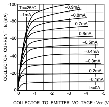
Fig.9 Grounded emitter output characteristics (I)
