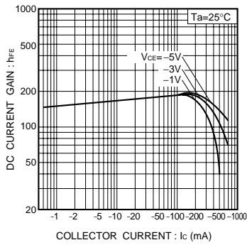
Fig.11 DC current gain vs. collector current (I)
