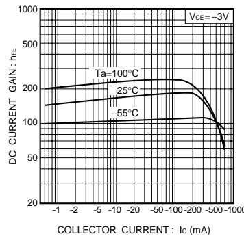
Fig.12 DC current gain vs. collector current (II)
