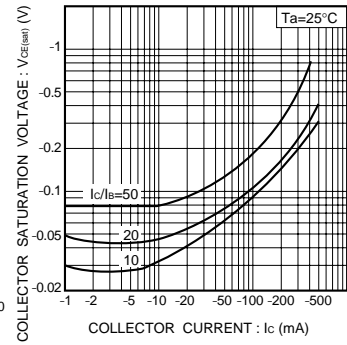
Fig.13 Collector-emitter saturation voltage vs. collector current (I)
