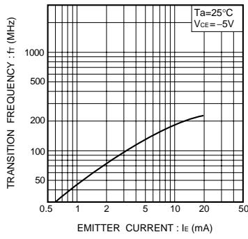
Fig.15 Gain bandwidth product vs. emitter current
