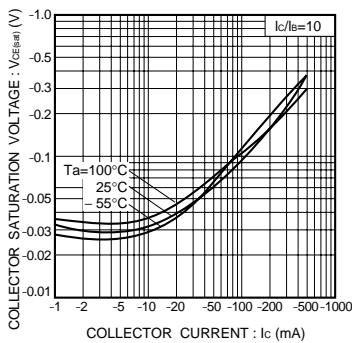
Fig.14 Collector-emitter saturation voltage vs. collector current (II)
