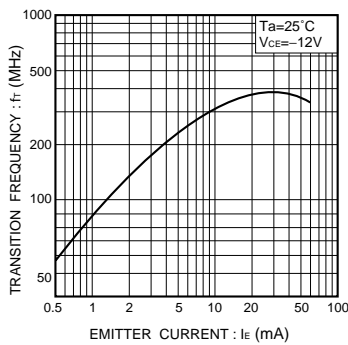
Fig.19 Gain bandwidth product vs. emitter current
