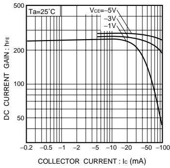
Fig.15 DC current gain vs. collector current ( I )
