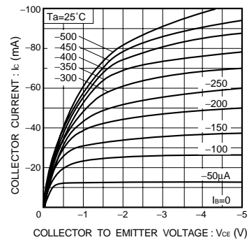
Fig.14 Grounded emitter output characteristics ( II )
