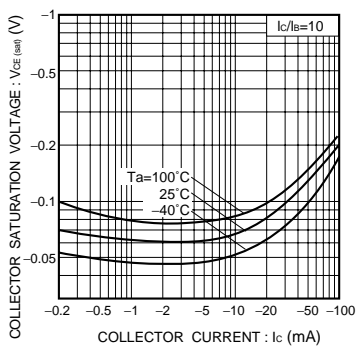
Fig.18 Collector-emitter saturation voltage vs. collector current ( II )
