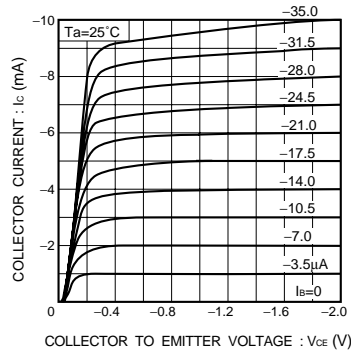
Fig.13 Grounded emitter output characteristics ( I )
