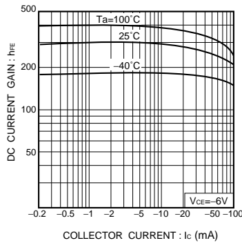
Fig.16 DC current gain vs. collector current ( II )
