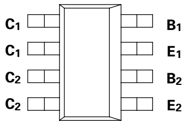
PARTMARKING DETAIL - T694
