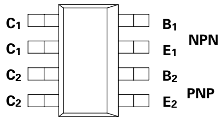
PARTMARKING DETAIL - T6718
