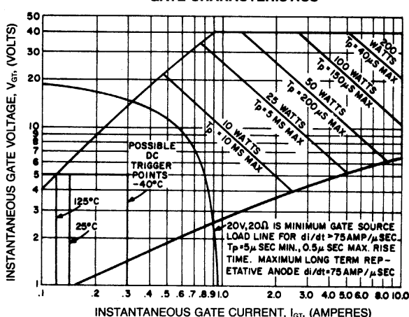
GATE CHARACTERISTICS
