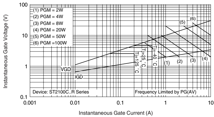
Fig. 11 - Gate Characteristics
