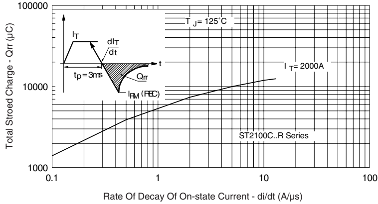
Fig. 7 - Stored Charged
