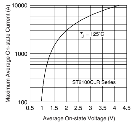
Fig. 4 - On-state Voltage Drop Characteristics
