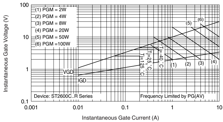
Fig. 11 - Gate Characteristics
