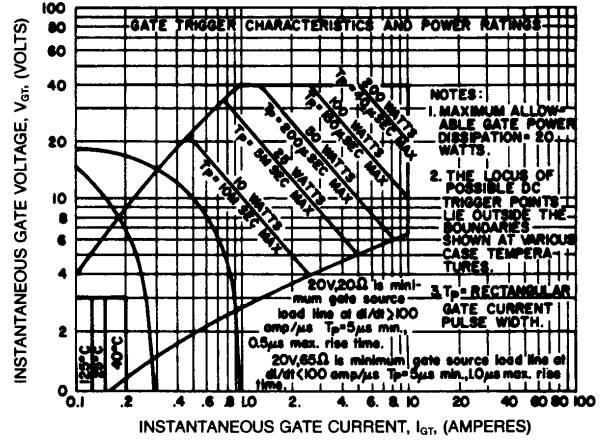
GATE CHARACTERISTICS
