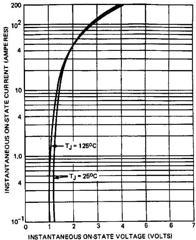
Fig. 2 – Maximum On-State Voltage Vs. Current, 2N681 Series
