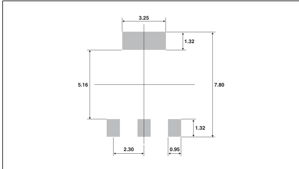
Figure 14. SOT-223 footprint
