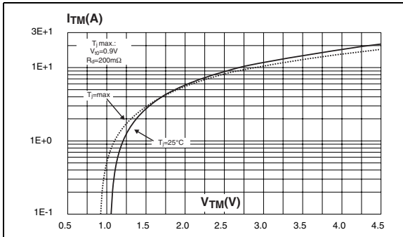
Figure 11. On-state characteristics (maximum values)
