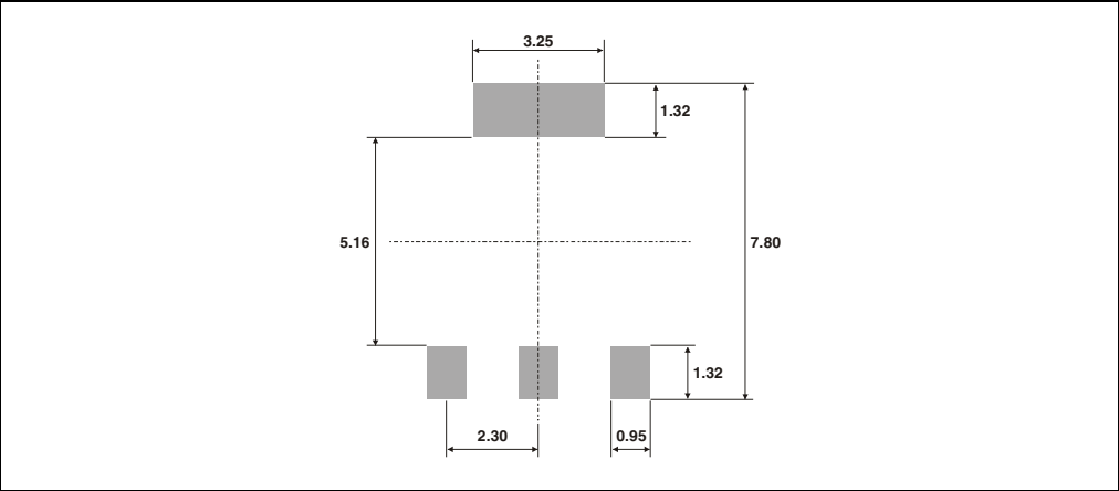
Figure 17. SOT-223 footprint (dimensions in mm)t
