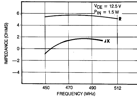
SERIES COLLECTOR LOAD IMPEDANCE VS FREQUENCY
