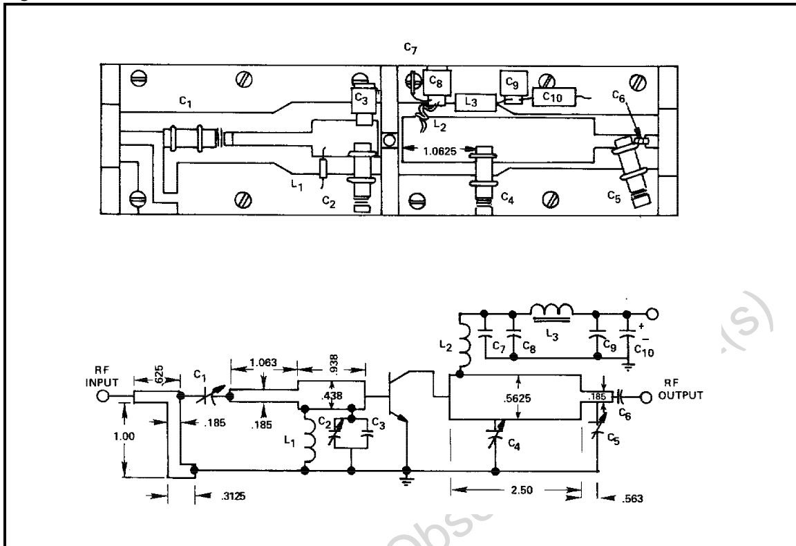
Figure 8. Test Circuit
