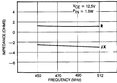
SERIES SOURCE IMPEDANCE VS FREQUENCY
