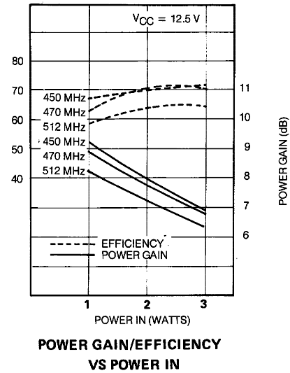
Figure 4. Power Gain &amp; Efficiency vs Power Input
