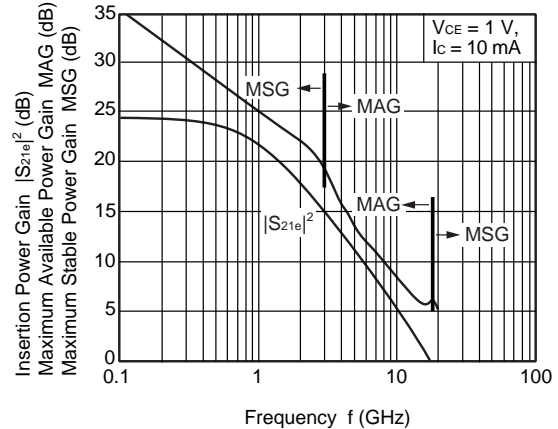
INSERTION POWER GAIN, MAG, MSG vs. FREQUENCY
