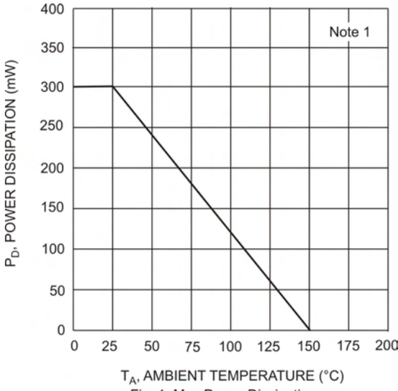
Fig. 1, Max Power Dissipation vs Ambient Temperature
