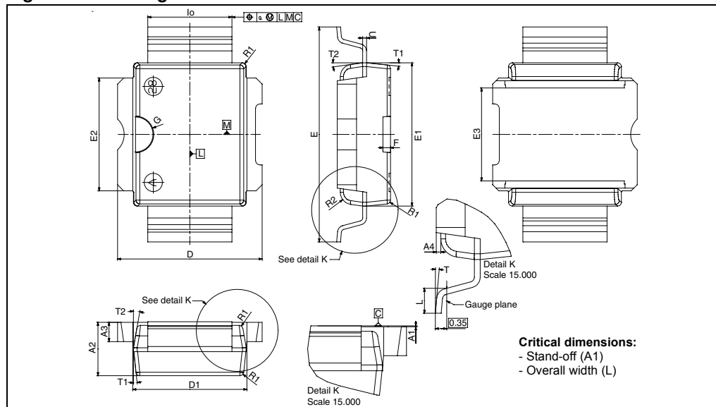
Figure 18. Package dimensions
