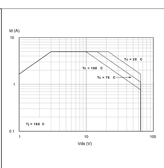
Figure 6. Safe operating area
