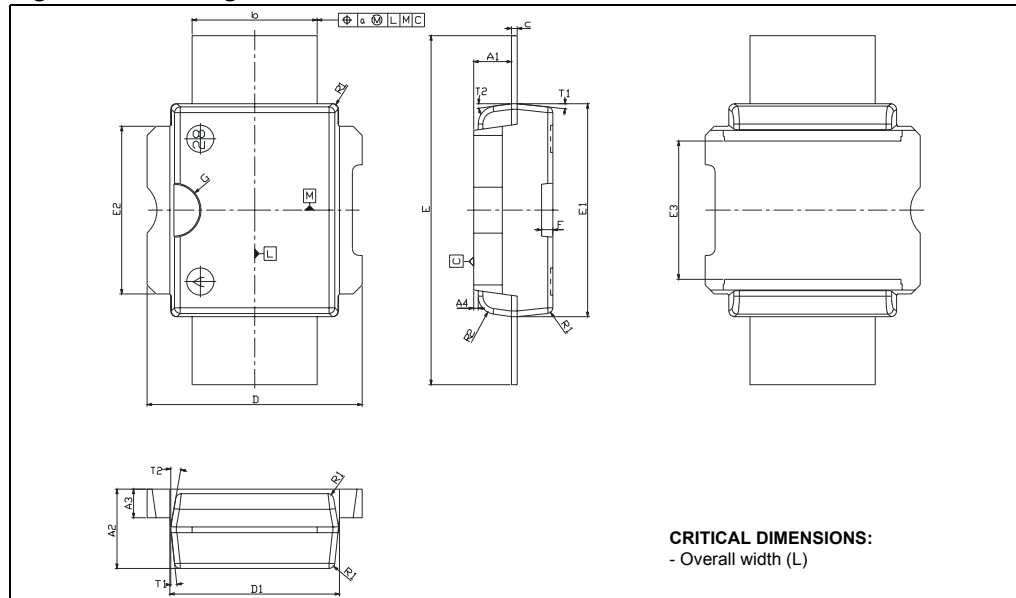
Figure 19. Package dimensions
