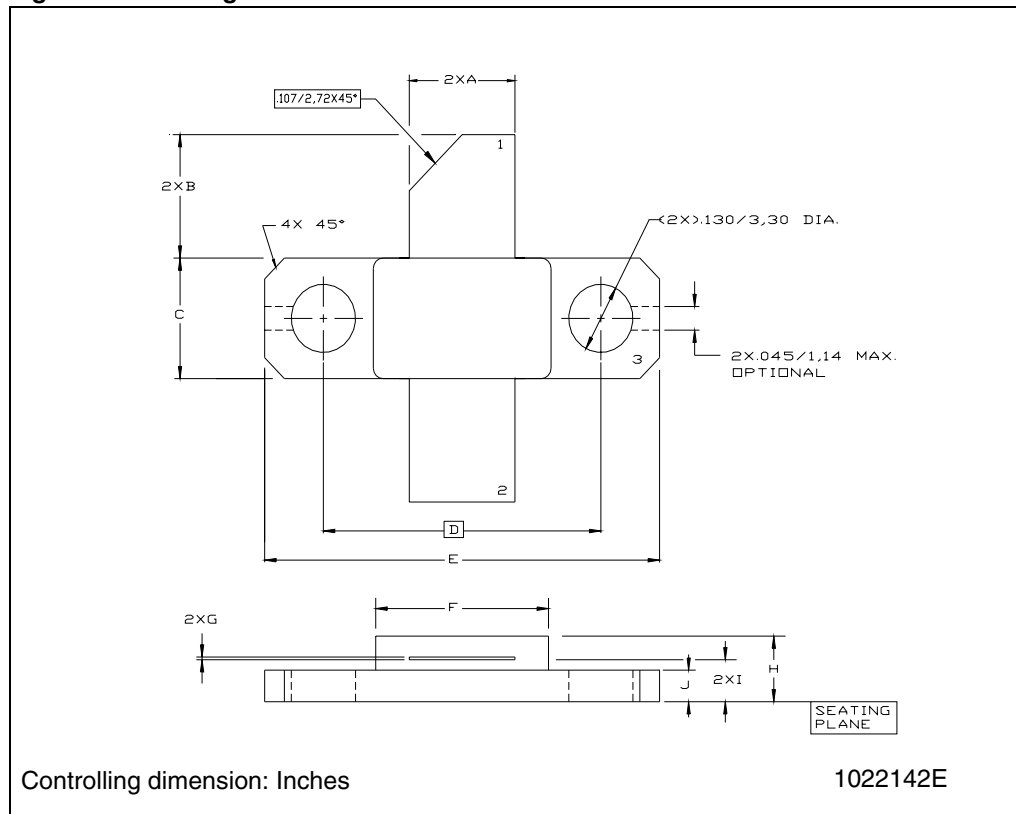
Figure 9. Package dimensions
