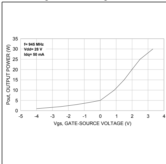
Figure 4. Output power vs gate source voltage
