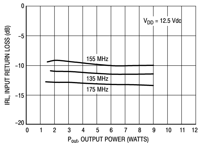
Figure 30. Input Return Loss versus Output Power
