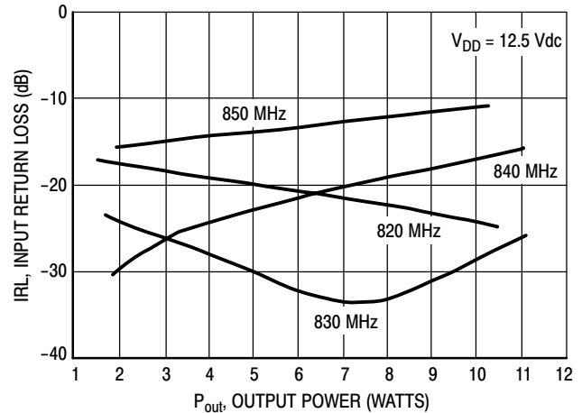
Figure 12. Input Return Loss versus Output Power
