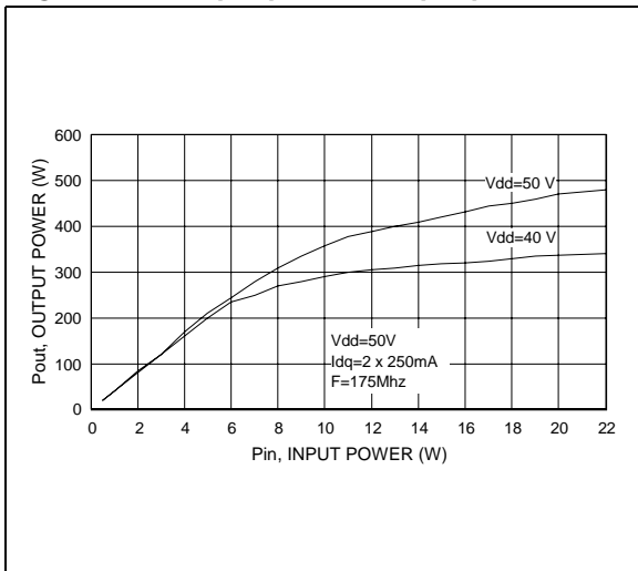
Figure 10. Output power vs input power
