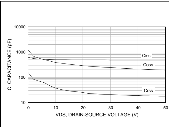
Figure 5. Capacitance vs drain-source voltage
