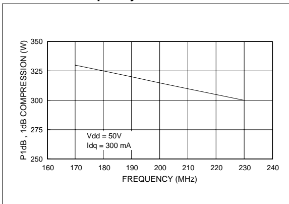
Figure 22. 1 dB compression point vs frequency
