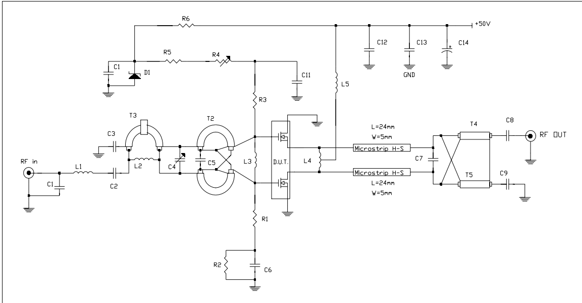
Figure 23. 175 - 230 MHz test circuit layout (engineering fixture)
