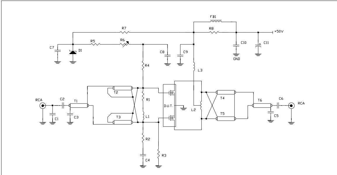
Figure 30. 88 - 108 MHz test circuit layout (engineering fixture)
