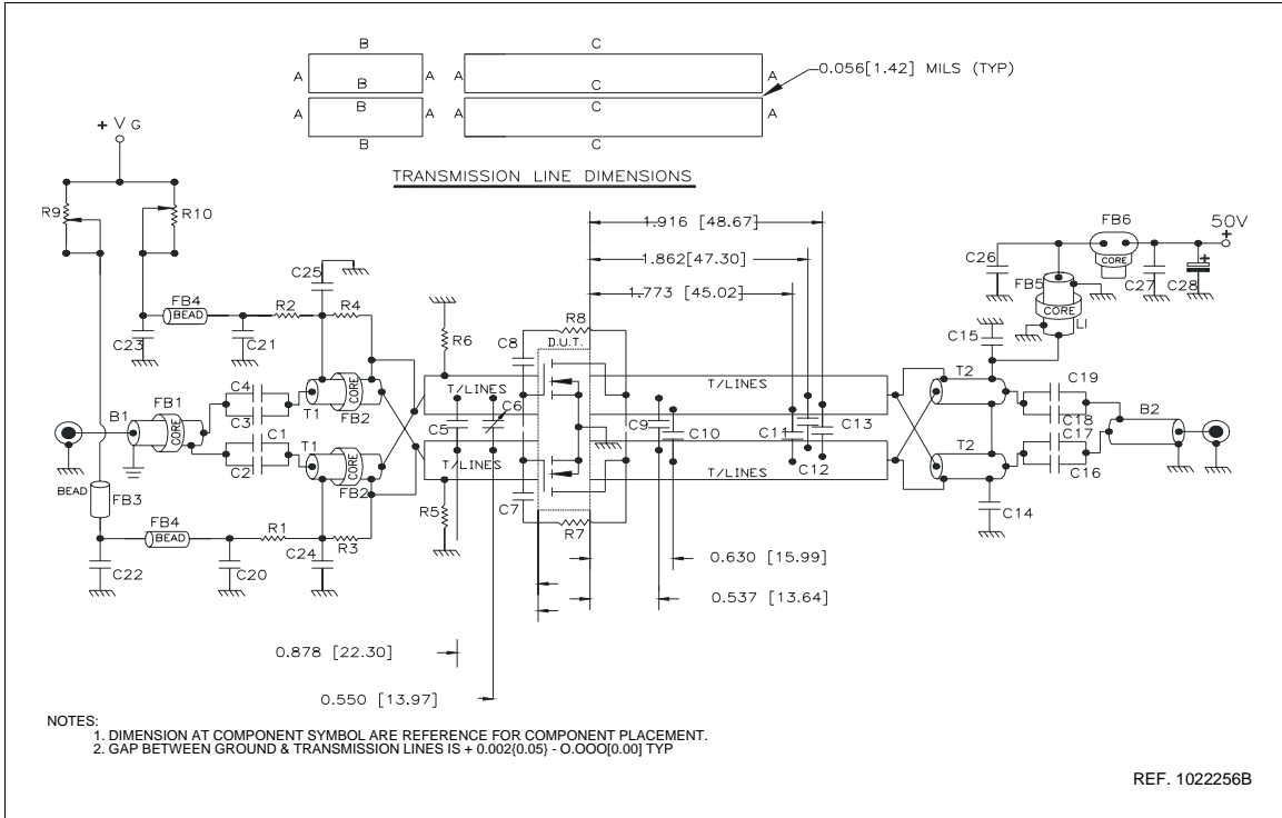
Figure 15. 175 MHz test circuit schematic (production test circuit
