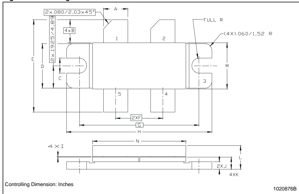
Figure 31. Package dimensions
