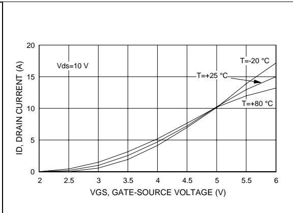
Figure 6. Drain current vs gate voltage
