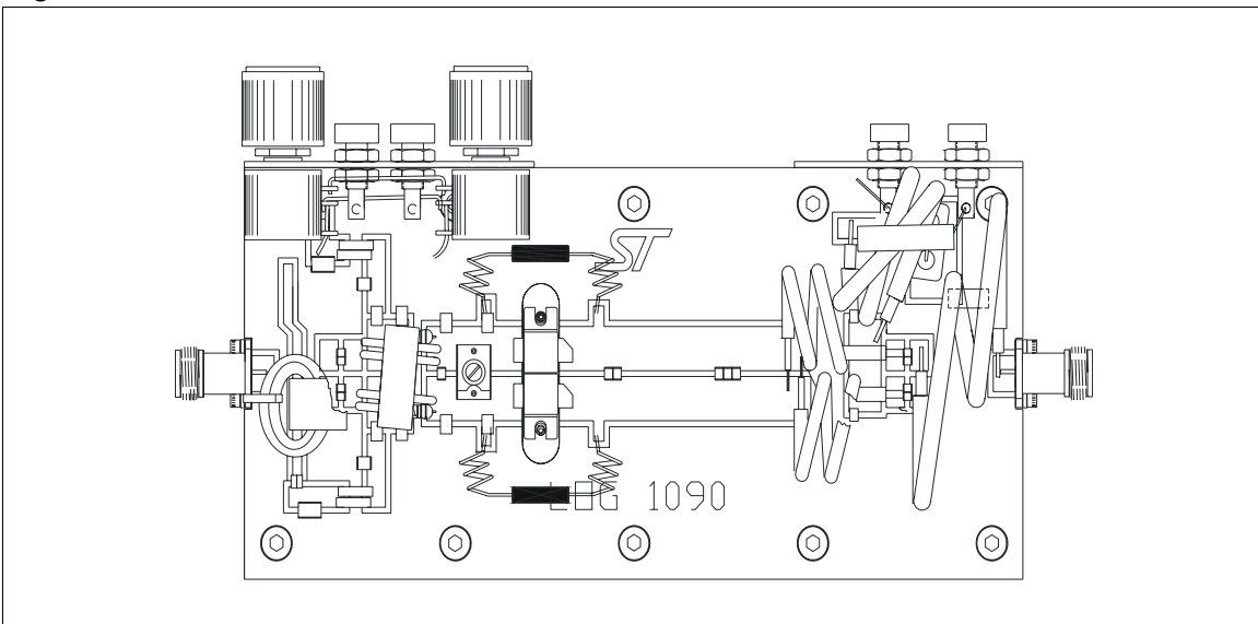
Figure 17. 175 MHz test fixture
