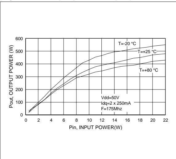
Figure 11. Output power vs input power
