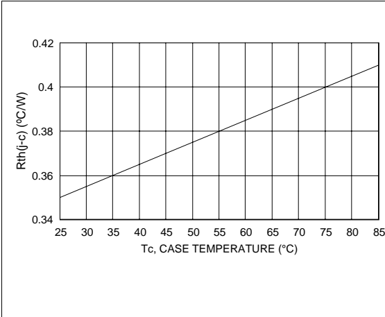
Figure 3. Maximum thermal resistance vs case temperature
