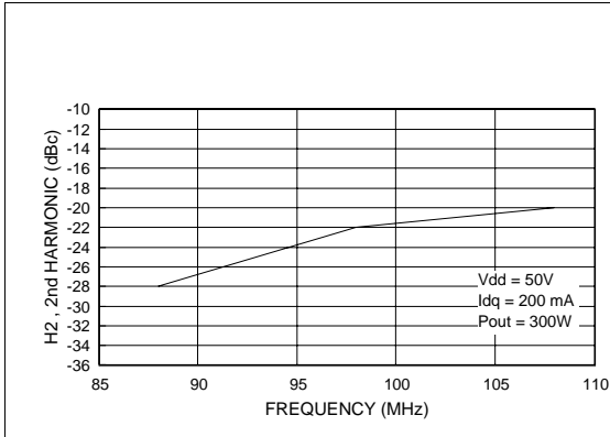
Figure 28. 2nd harmonic vs. frequency (88 - 108 MHz)
