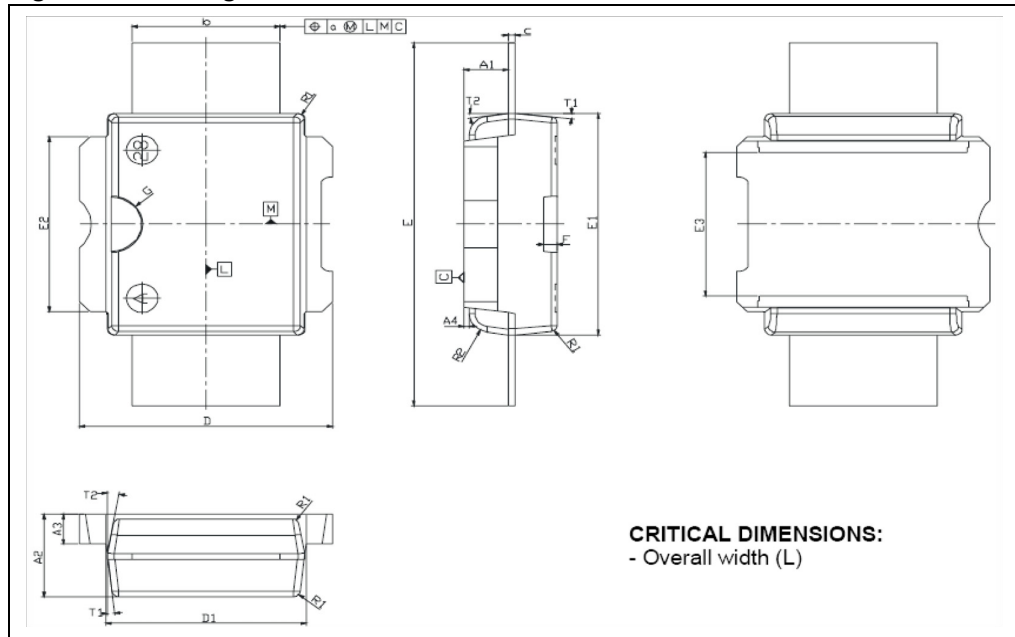
Figure 29. Package dimensions
