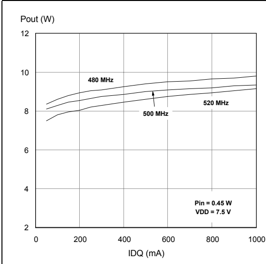
Figure 20. Output power vs. bias current
