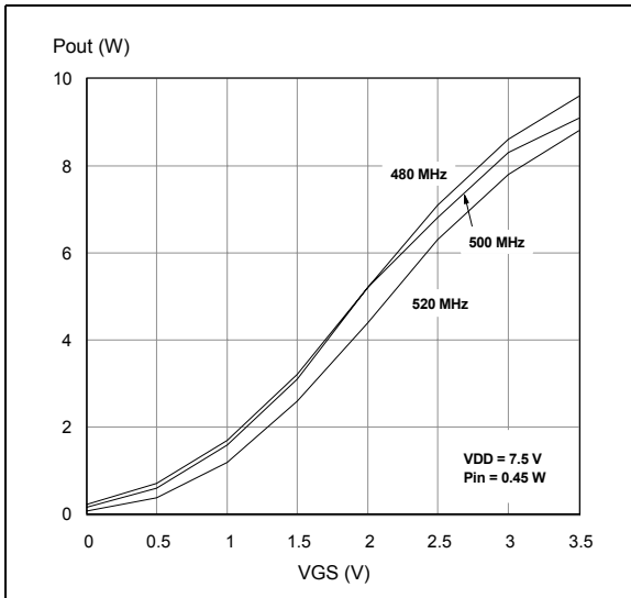
Figure 24. Output power vs. gate bias voltage
