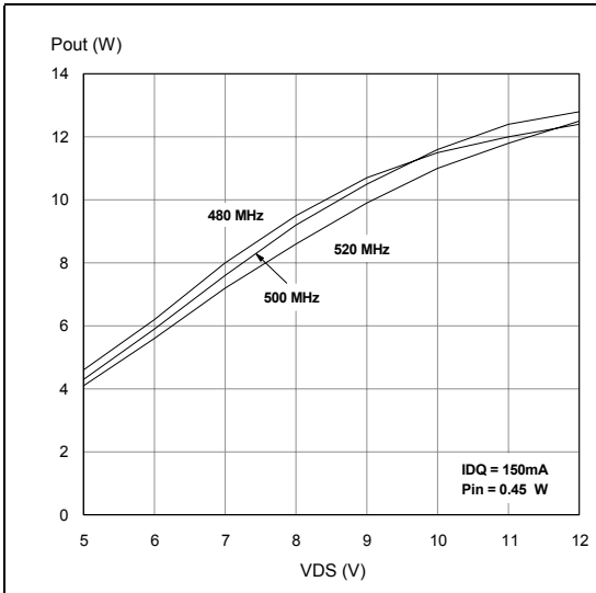
Figure 22. Output power vs. drain voltage
