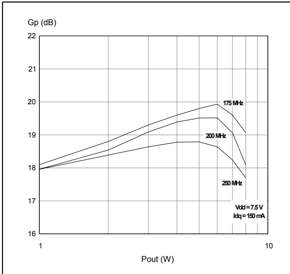
Figure 15. Power gain vs. output power
