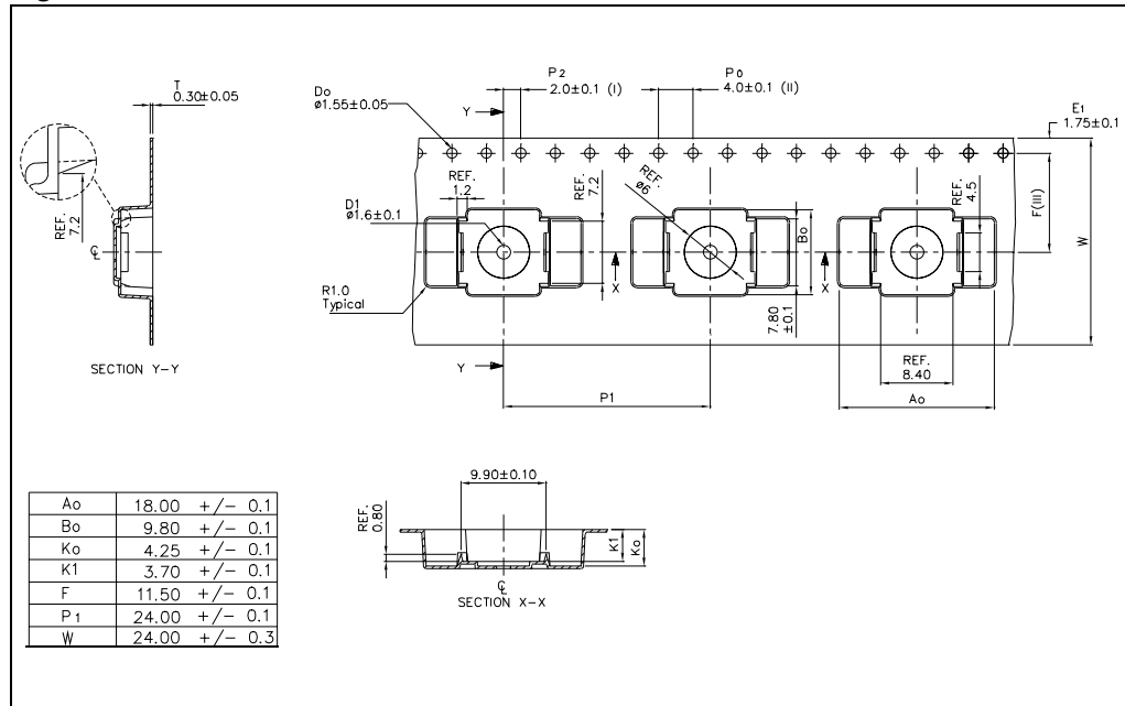
Figure 31. Reel information
