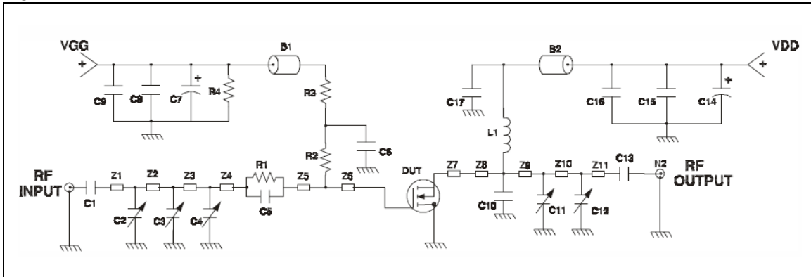
Figure 25. Test circuit schematic
