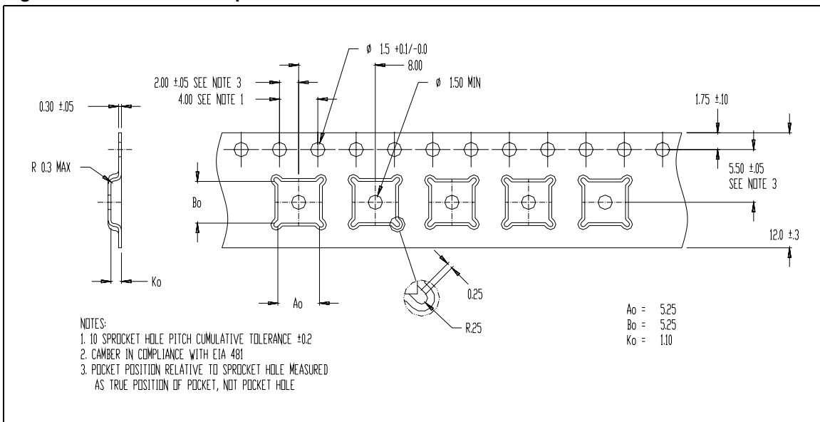
Figure 11. PowerFLAT™ tape & reel
