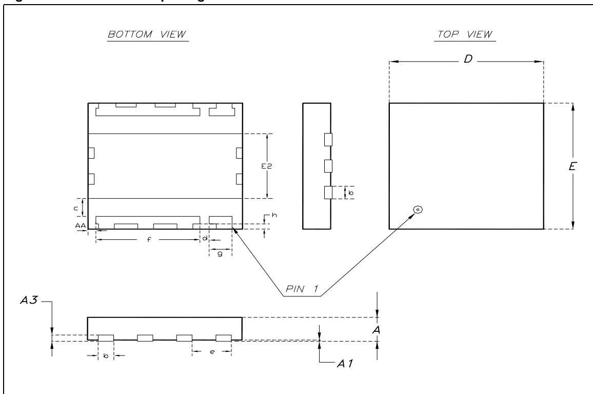
Figure 10. PowerFLAT™ package dimensions
