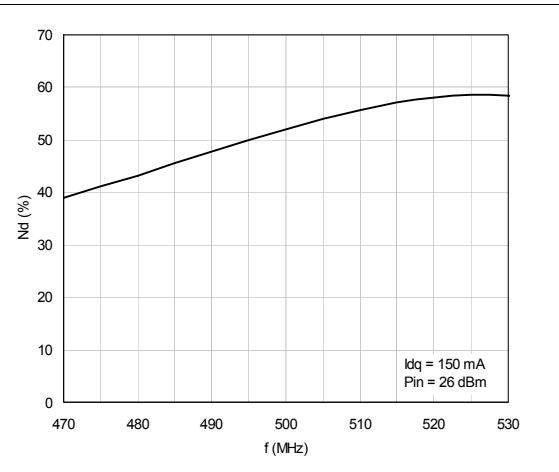
Figure 7. Efficiency vs frequency
