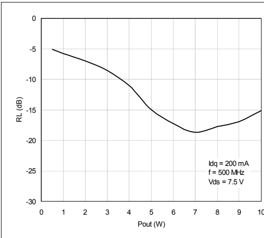
Figure 4. Return loss vs output power
