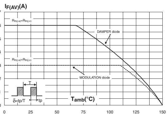
Figure 2: Average forward current versus ambient temperature
