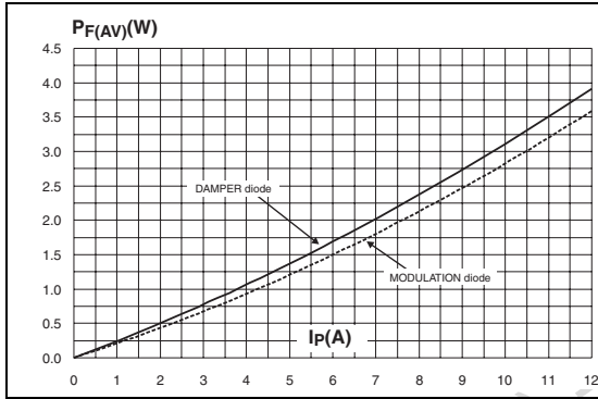
Figure 1. Power dissipation vs. peak forward current (triangular waveform, \delta = 0.45 )
