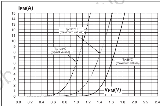
Figure 3. Forward voltage drop vs. forward current (damper diode)
