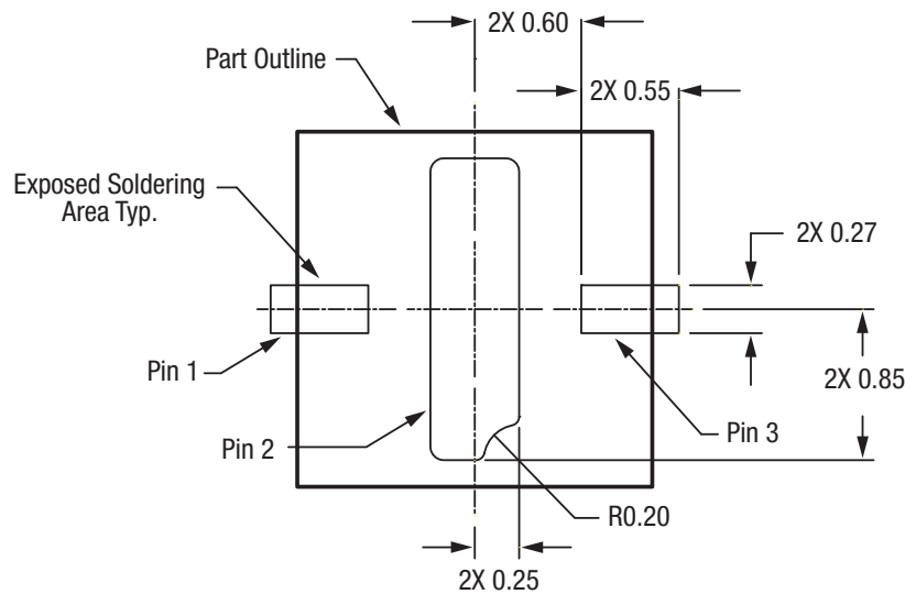
Figure 9. CLA4609-086LF PCB Layout Footprint
