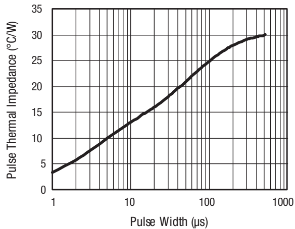
Figure 5. Typical Pulse Thermal Impedance
