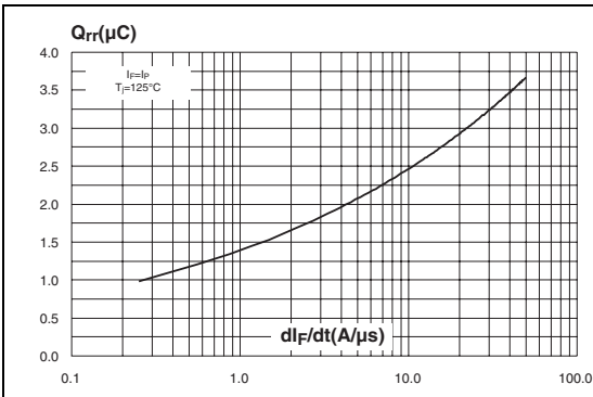
Figure 7. Reverse recovery charges vs. di_F/dt (damper diode)
