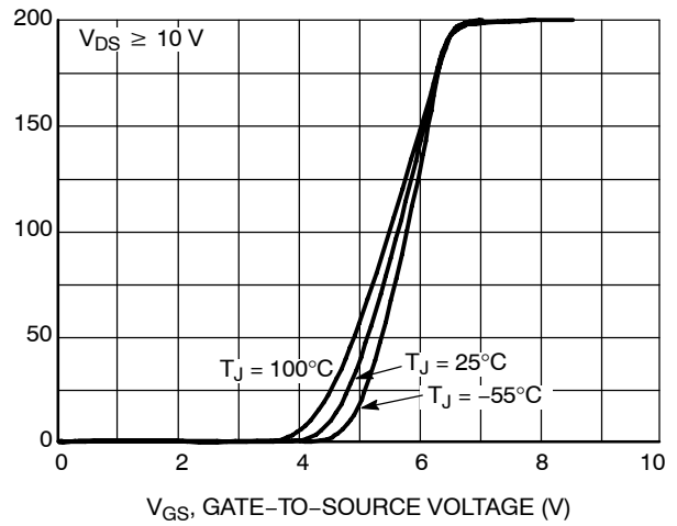
Figure 2. On-Region Characteristics
