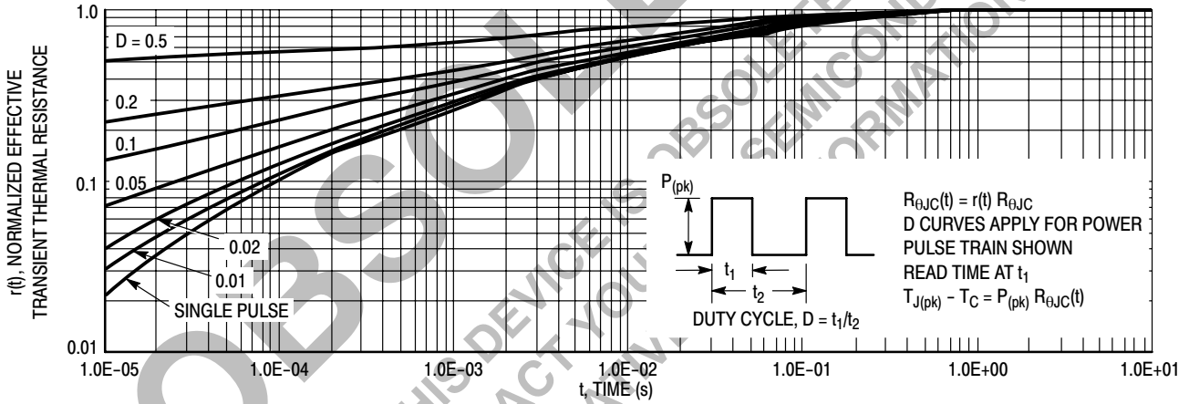
Figure 13. Thermal Response
