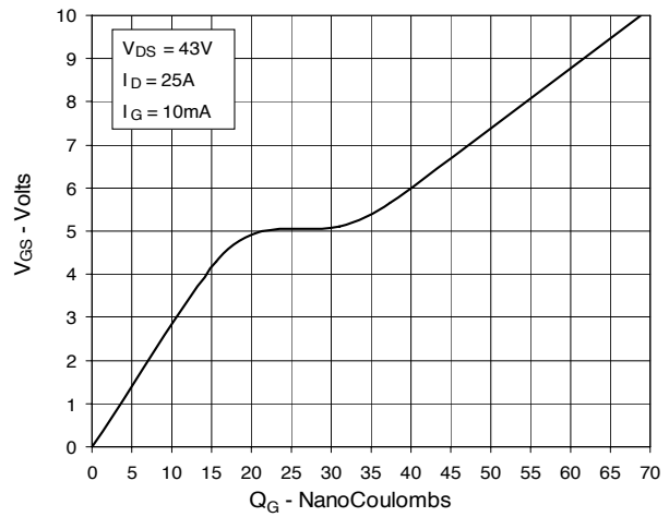
Fig. 10. Gate Charge
