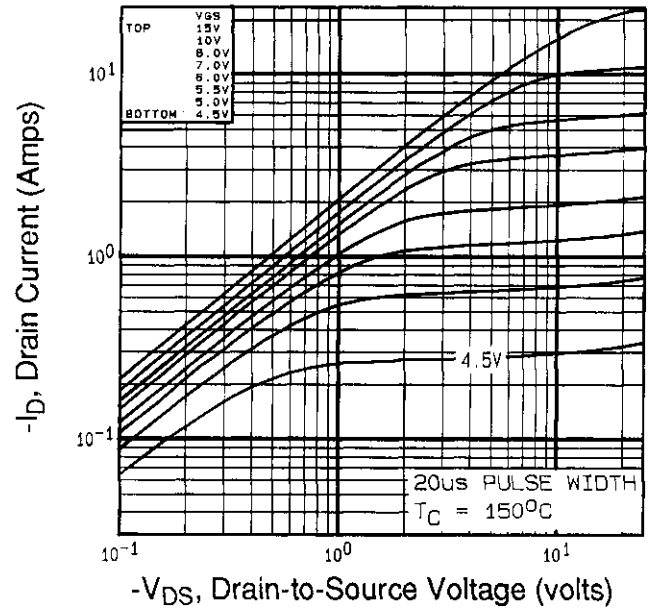
Fig 2. Typical Output Characteristics, T_C=150^\circ C
