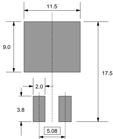
Fig.19. SOT404 : soldering pattern for surface mounting.
