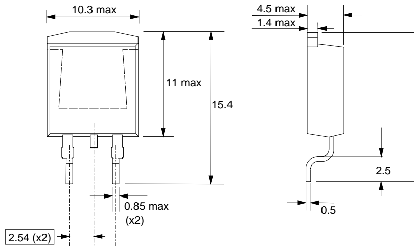
Fig.18. SOT404 : centre pin connected to mounting base.
