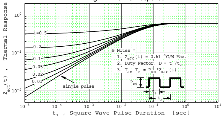
Fig 11. Thermal Response
