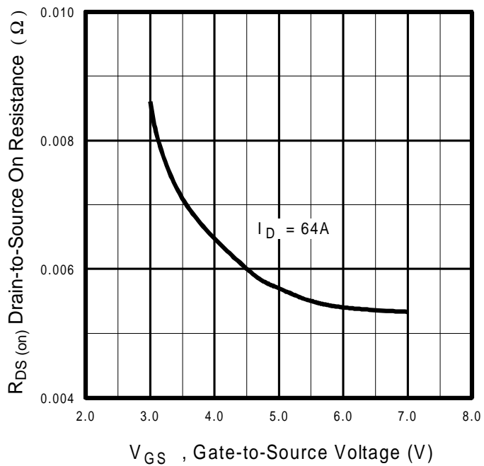
Fig 13. On-Resistance Vs. Gate Voltage
