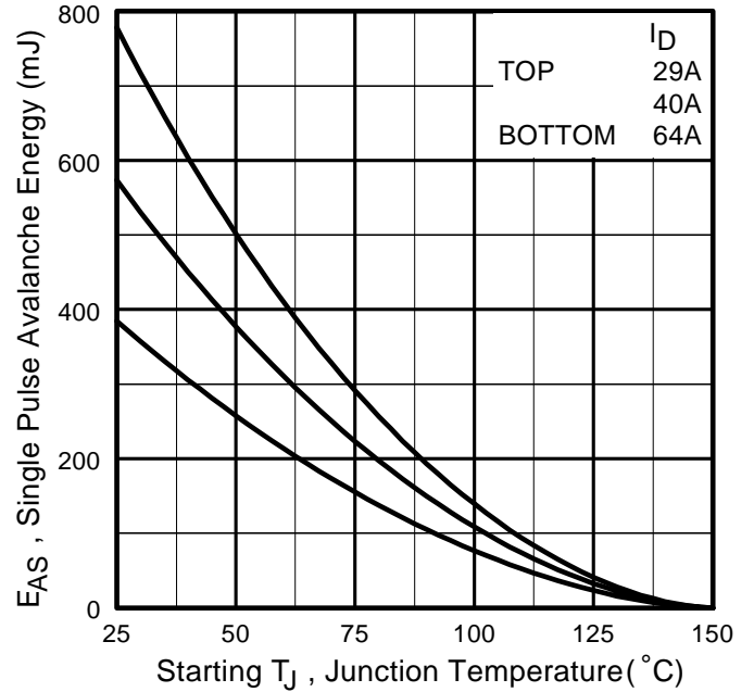
Fig 10. Maximum Avalanche Energy Vs. Drain Current
