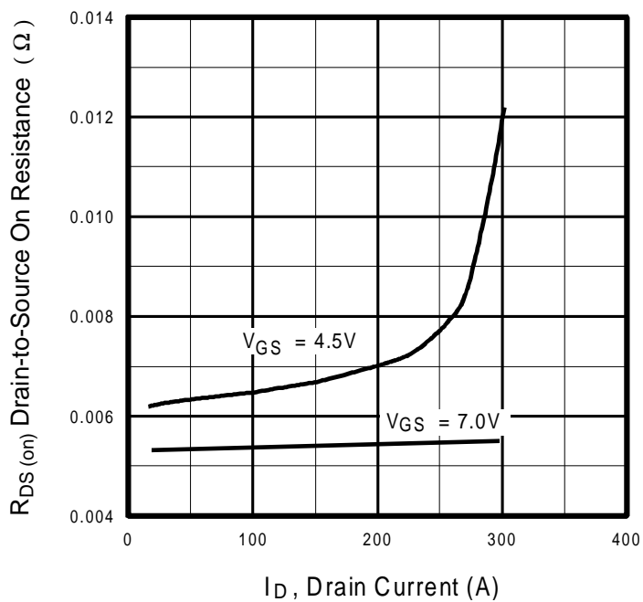
Fig 12. On-Resistance Vs. Drain Current
