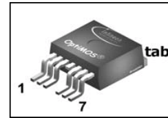
PG-TO263-7
