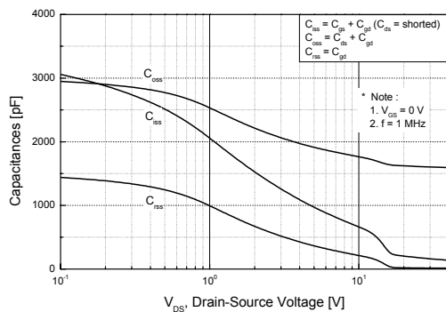
Figure 5. Capacitance Characteristics
