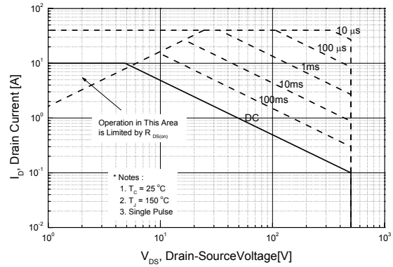
Figure 9-2. Maximum Safe Operating Area for FQPF10N50CF
