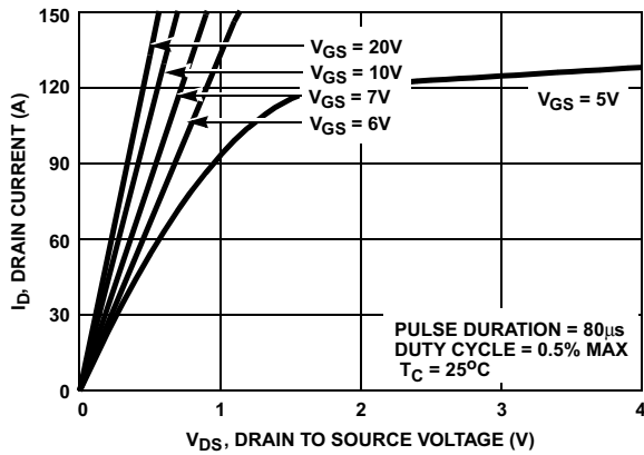
FIGURE 7. SATURATION CHARACTERISTICS
