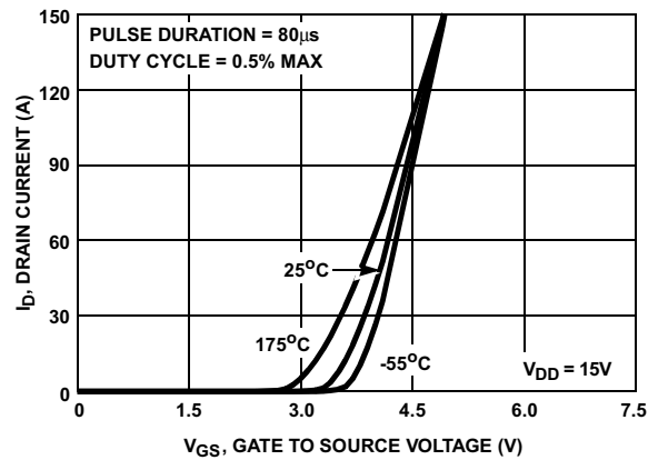
FIGURE 8. TRANSFER CHARACTERISTICS
