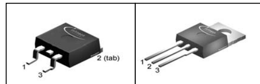
PG-TO263-3-2
