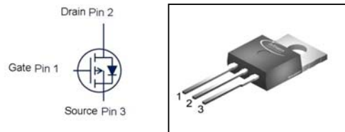
PG-TO220-3
