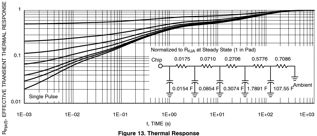
Figure 13. Thermal Response
