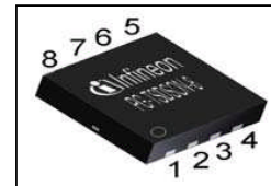
PG-TSDSON-8
