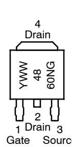
1 Gate 2 Drain 3 Source
