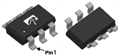
TSOP6 Top View Bottom View
