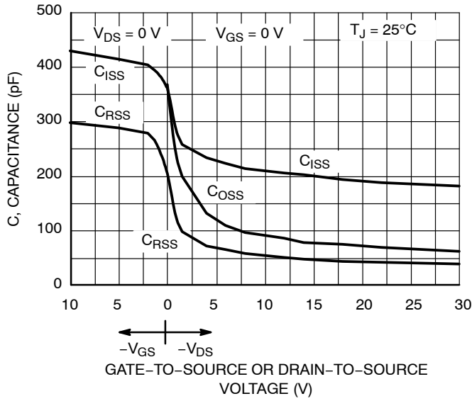
Figure 7. Capacitance Variation
