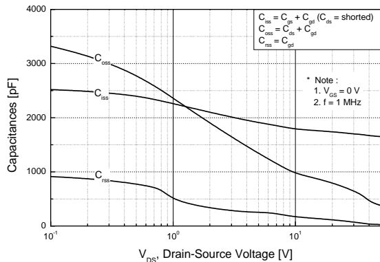
Figure 5. Capacitance Characteristics
