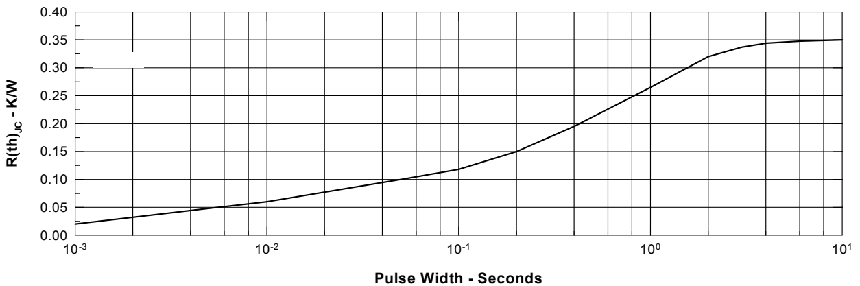
Figure 11. Transient Thermal Resistance
