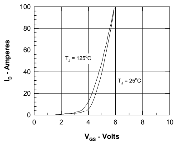
Figure 6. Admittance Curves
