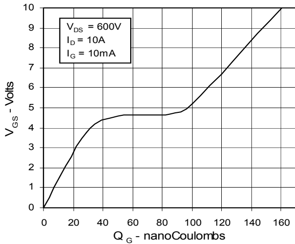
Fig. 9. Gate Charge
