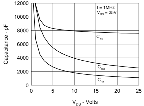
Fig.8 Capacitance Curves
