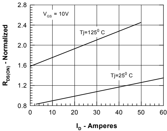
Figure 3. R_{DS(on)} normalized to 15A/25°C vs. I_D
