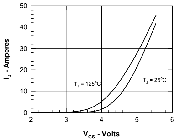
Figure 6. Admittance Curves
