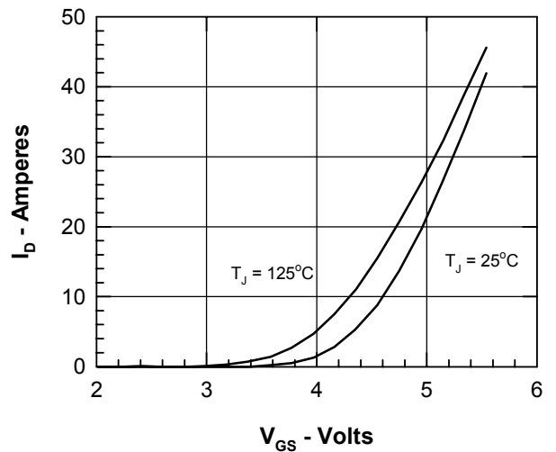
Figure 6. Admittance Curves
