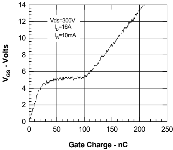
Figure 7. Gate Charge
