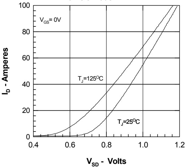
Figure 9. Forward Voltage Drop of the Intrinsic Diode
