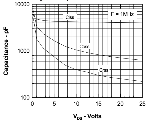
Figure 8. Capacitance Curves
