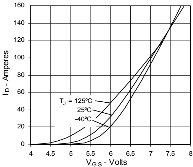
Fig. 7. Input Admittance
