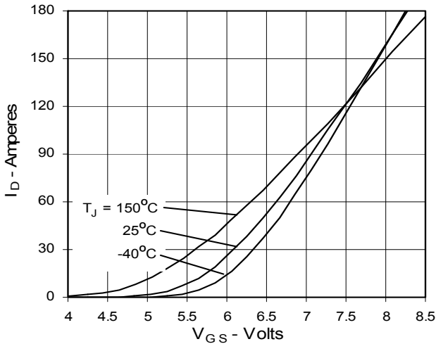
Fig. 7. Input Admittance
