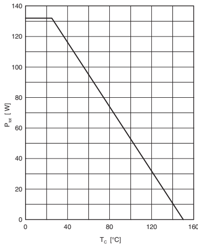
Fig. 1 Power dissipation
