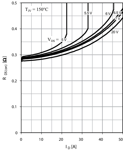
Fig. 4 Typ. drain-source on-state resistance
