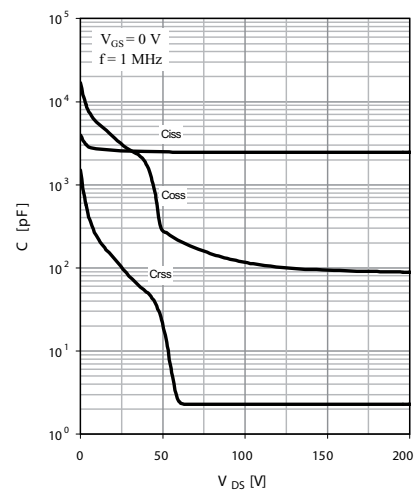
Fig. 9 Typ. capacitances
