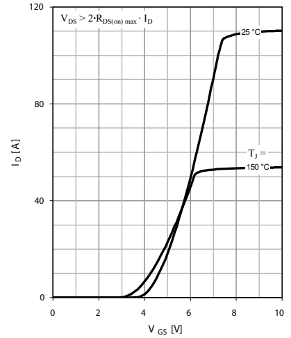
Fig. 6 Typ. transfer characteristics
